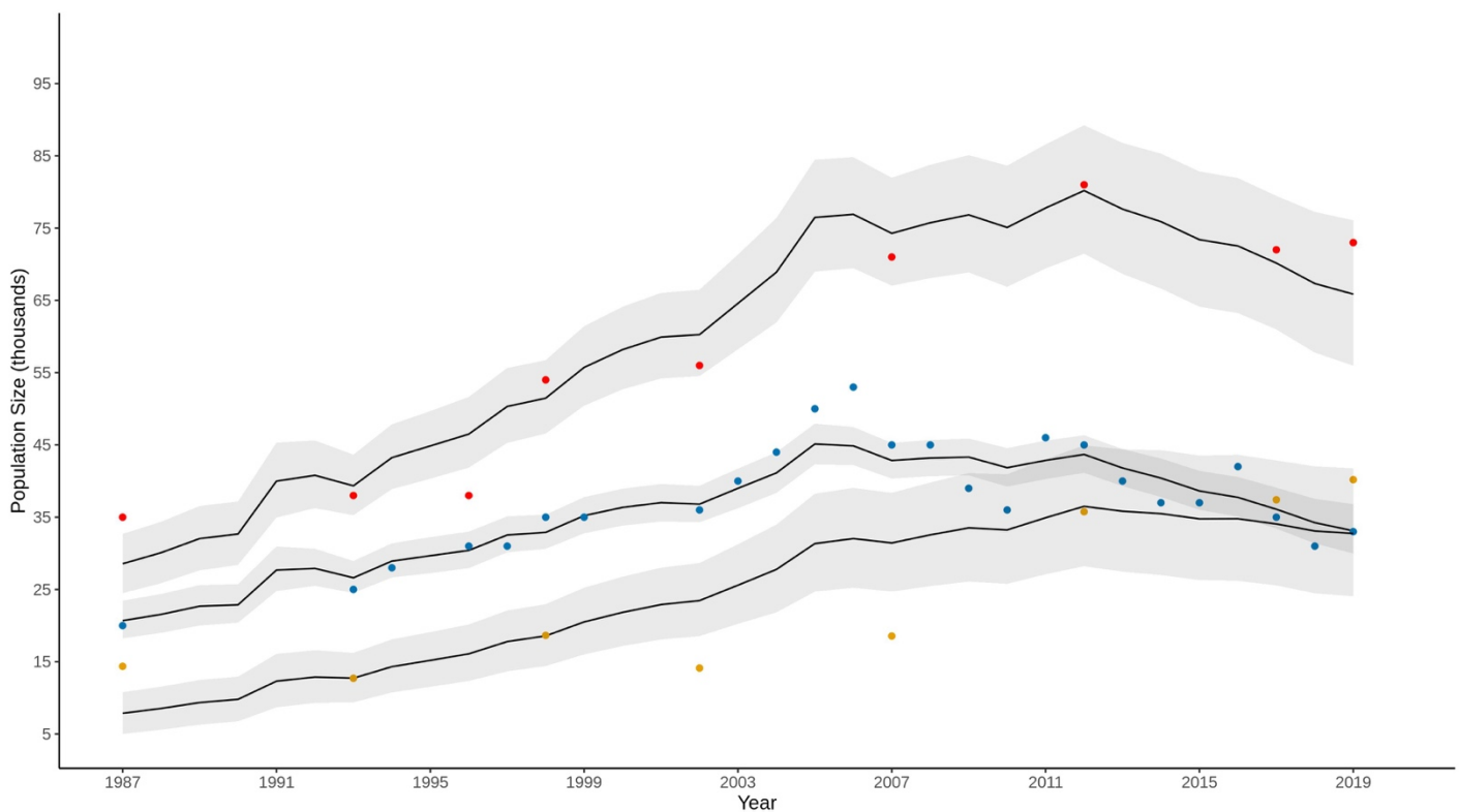
Figure 8. Posterior estimates of Greenland Barnacle Goose population size (in thousands) in black with 95% credible intervals shown in grey. Data-based counts (in thousands) are shown as points for the total flyway (red), Islay (blue), other (yellow).
