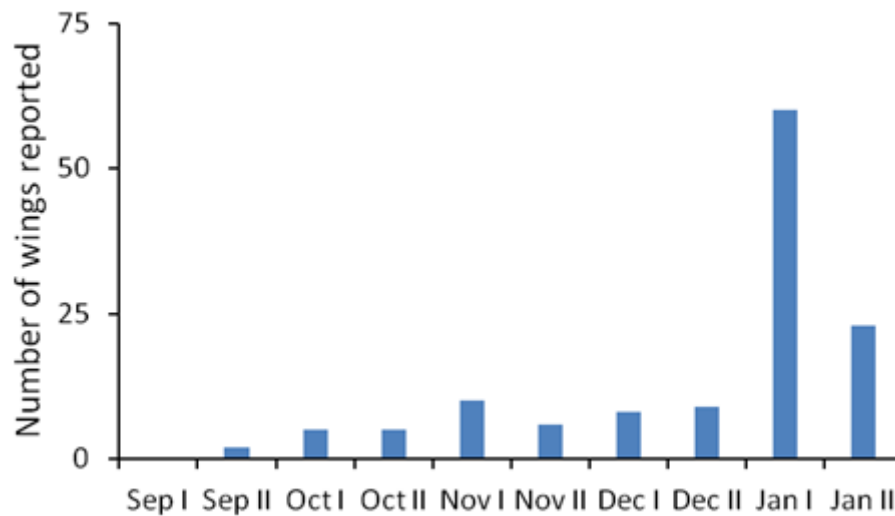
Figure 6. Number of wings of Pink-footed Geese ( N_{\text{total}}=128 ) collected from hunters in Denmark in the 2019/20 hunting season, divided into half-monthly intervals.
