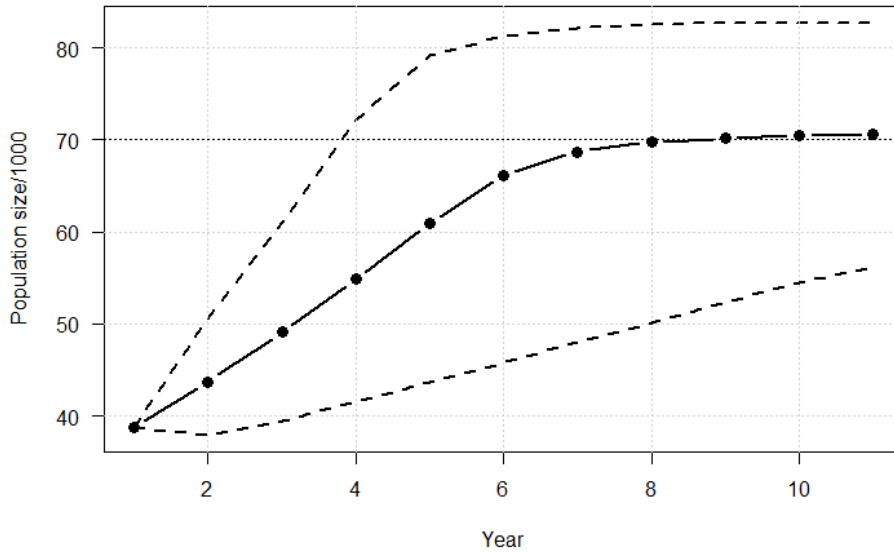
Figure 6. Simulated population sizes (median and 95% confidence limits) of taiga bean geese in the Central Management using a dynamic harvesting strategy with a sole objective of maintaining the population near the goal of 70,000 birds in January.
