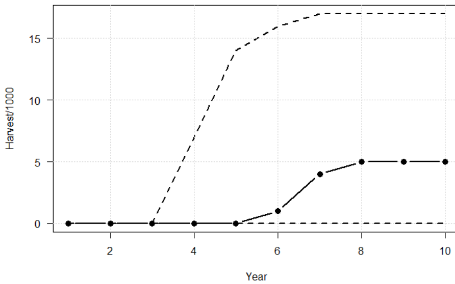
Figure 8. Simulated harvests (median and 95% confidence limits) of taiga bean geese in the Central Management using a dynamic harvesting strategy with a sole objective of maintaining the population near the goal of 70,000 birds in January
