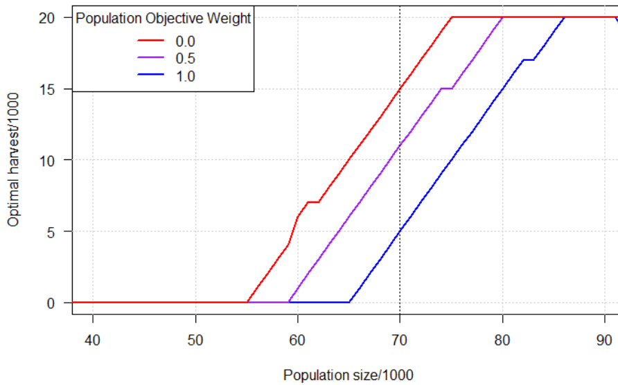
Figure 11. Dynamic harvest strategies for the Central Management Unit of taiga bean geese. The three strategies have different weights on the objective to maintain the population around 70,000 birds in January. The weight on the objective of sustainable harvest is the complement of the population objective weight.
