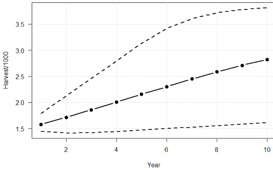
Figure 7. Simulated harvest quotas (median and 95% confidence limits) of taiga bean geese in the Central Management, given a target adult harvest rate h_a = 0.03
