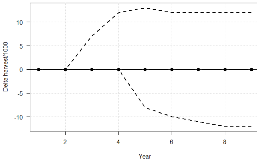
Figure 10. Simulated annual differences in harvest quotas (median and 95% confidence limits) of taiga bean geese in the Central Management using a dynamic harvesting strategy with a sole objective of maintaining the population near the goal of 70,000 birds in January.
