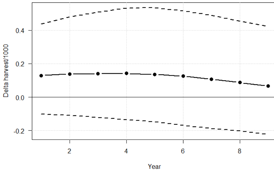
Figure 9. Simulated annual differences in harvest quotas (median and 95% confidence limits) of taiga bean geese in the Central Management, given a target adult harvest rate h_a = 0.03
