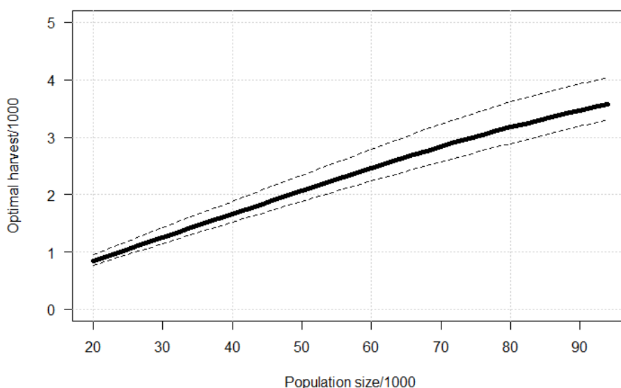
Figure 3. Median harvest quotas and 95% confidence limits for a range of taiga bean goose population sizes in the Central Management Unit in January based on a target adult harvest rate h_a = 0.03
