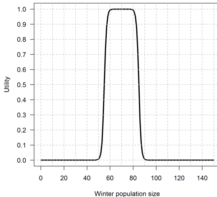
Figure 2. Possible utility of mid-winter population sizes of taiga bean geese in the Central Management Unit
