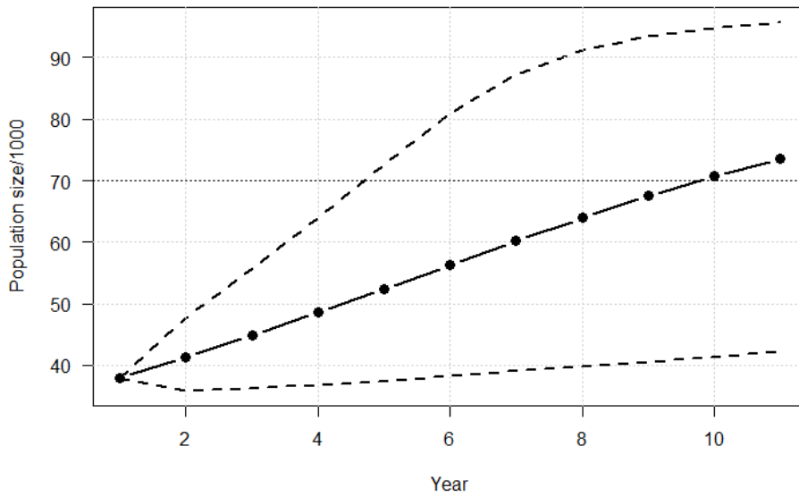
Figure 5. Simulated population sizes (median and 95% confidence limits) of taiga bean geese in the Central Management, given a target adult harvest rate h_a = 0.03 . The dotted horizontal line indicates the population goal of 70,000 birds in January.
