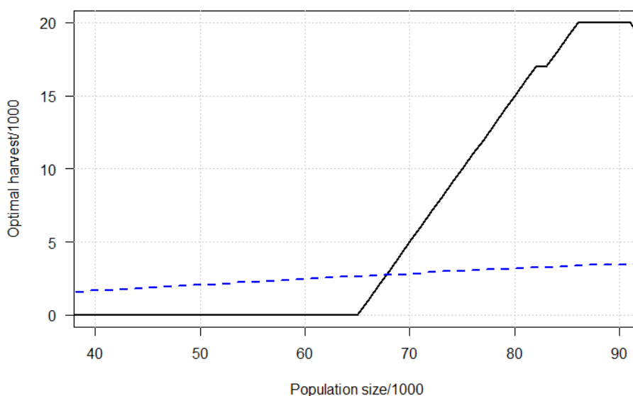
Figure 4. A dynamic harvest strategy (black solid line) design to maintain the population near its goal compared to the constant harvest-rate strategy with a target adult harvest rate h_a = 0.03 (blue dashed line) for the Central Management Unit of Taiga Bean Geese
